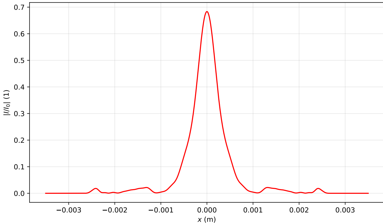
Intensity profile I(x, y = 0, z = 3.105)/I_0 , P_{in}=3.5P_{cr} , artificial time
